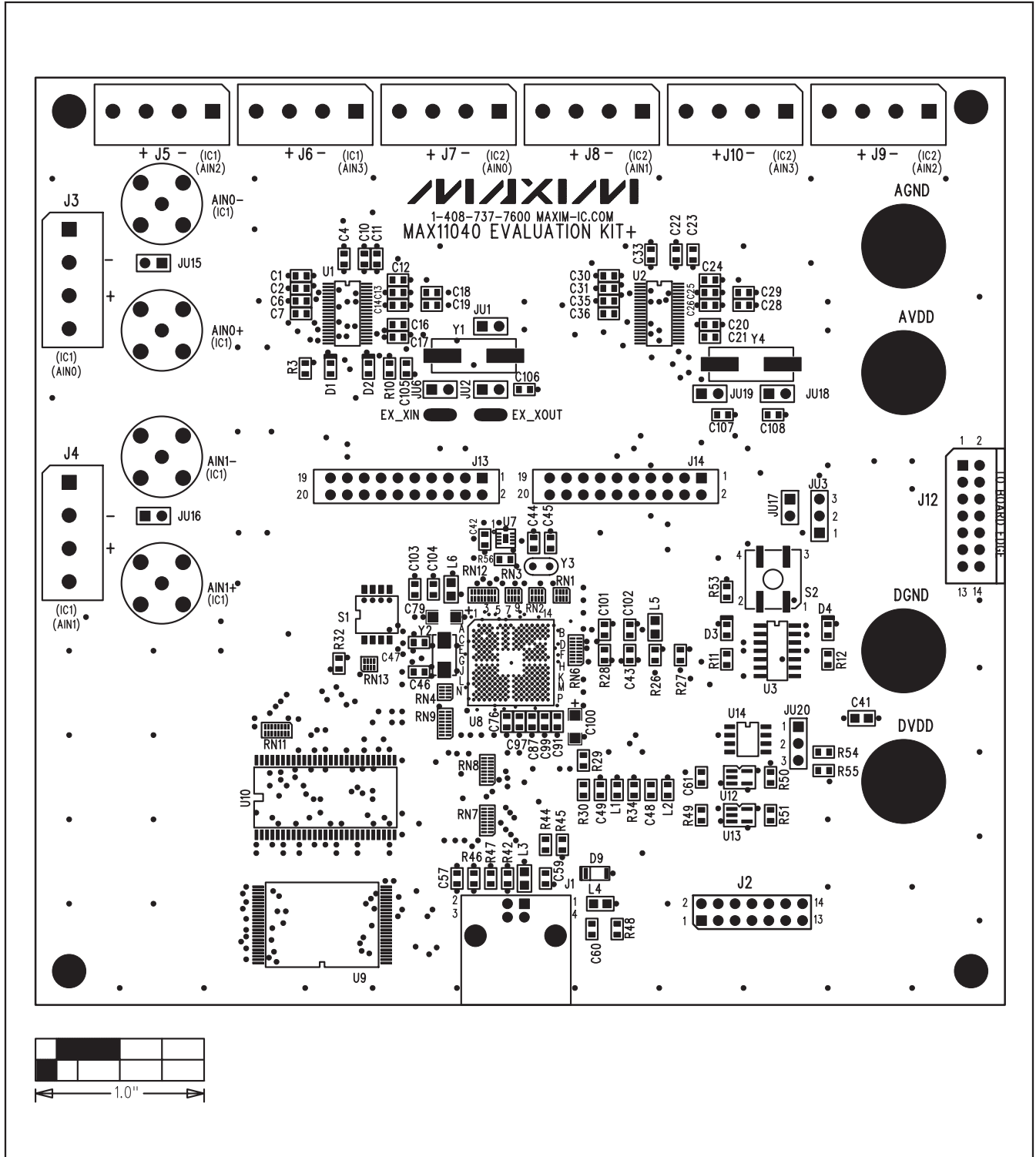
Figure 3. MAX11040 EV Kit Component Placement Guide—Top
