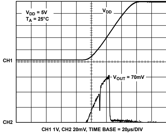
Figure 17. Power-On Reset to 0V
