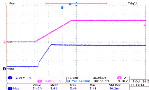
Power On Response: HT7550-7 ( I_{OUT}=0mA , T_{RISE}=100ms )
