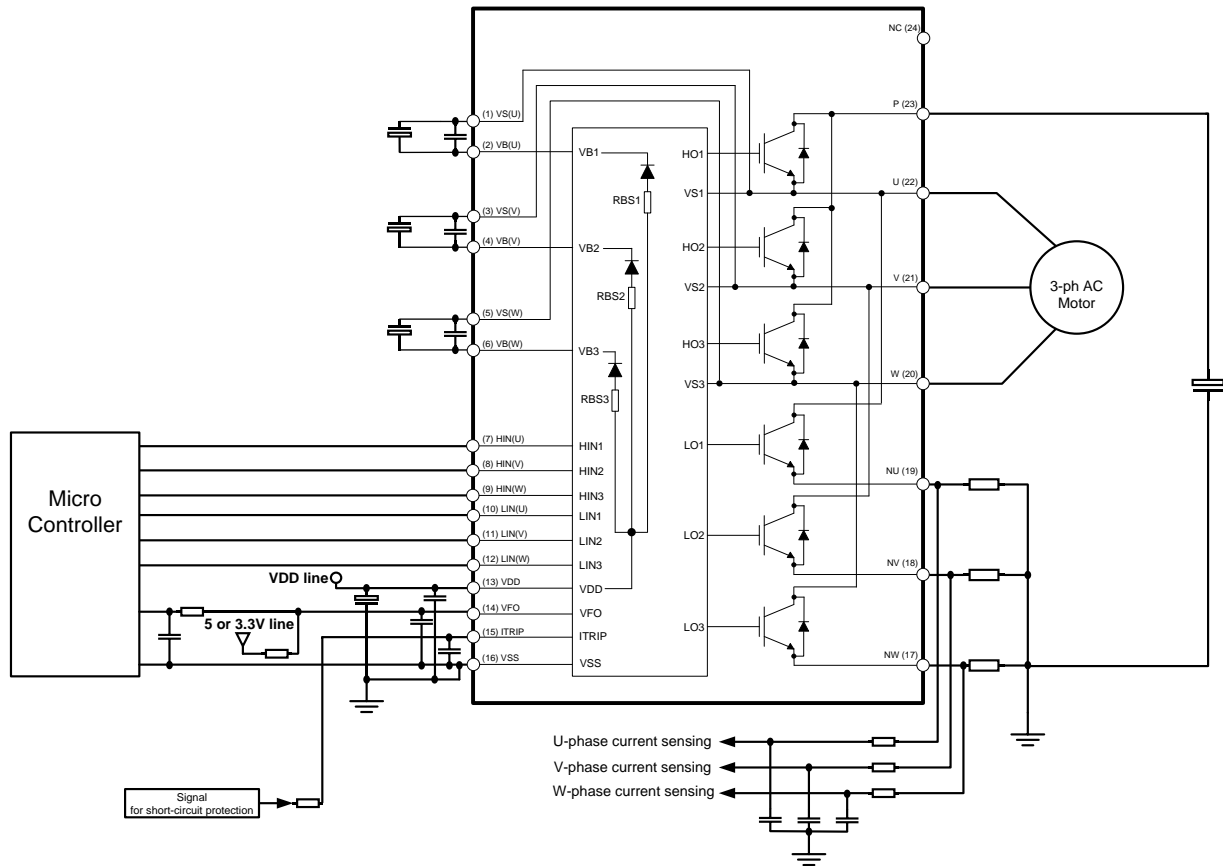
Figure 8: Application circuit
