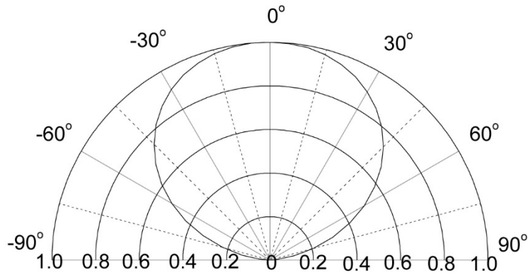
Figure3. Relative Luminosity VS. Radiation Angle
