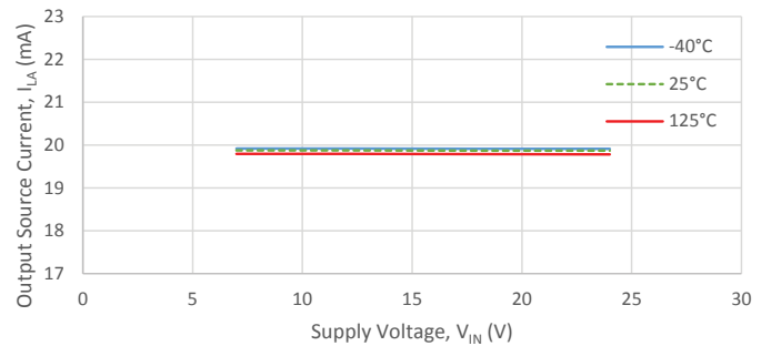
Output Source Current ( I_{LA} v. V_{IN} ) I_{REF} = 0.267 mA
