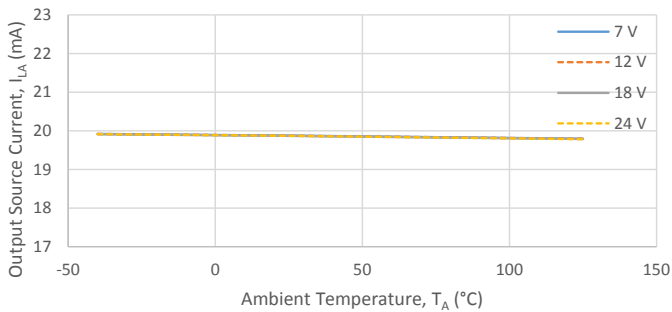
Output Source Current ( I_{LA} v. T_A ) I_{REF} = 0.267 mA
