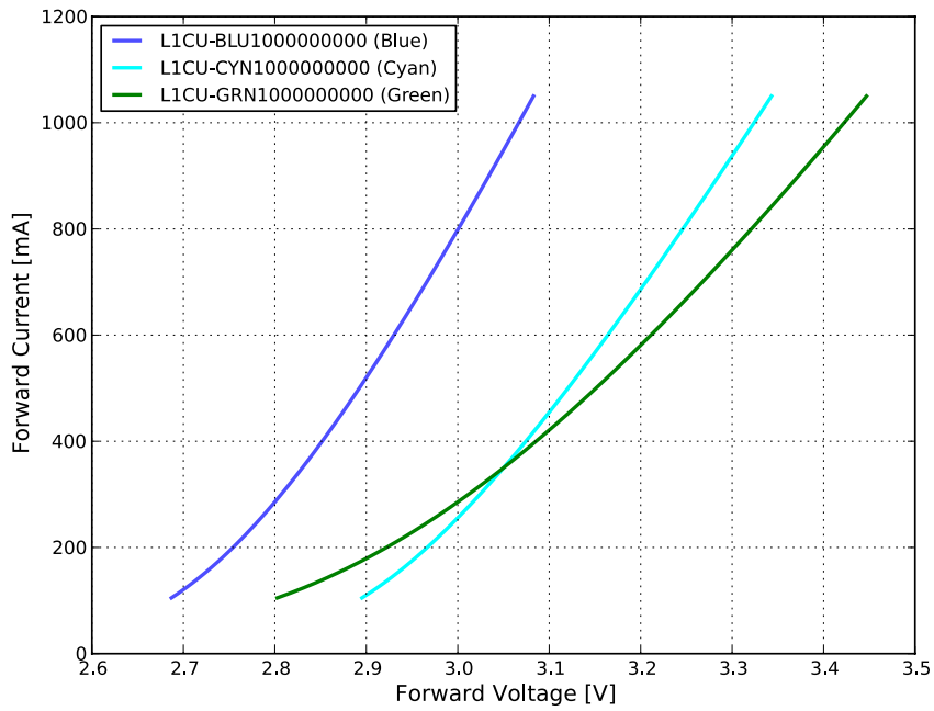
Figure 4d. Typical forward current vs. forward voltage for LUXEON CZ Green, Cyan and Blue at T_j=85^\circ\text{C} .
