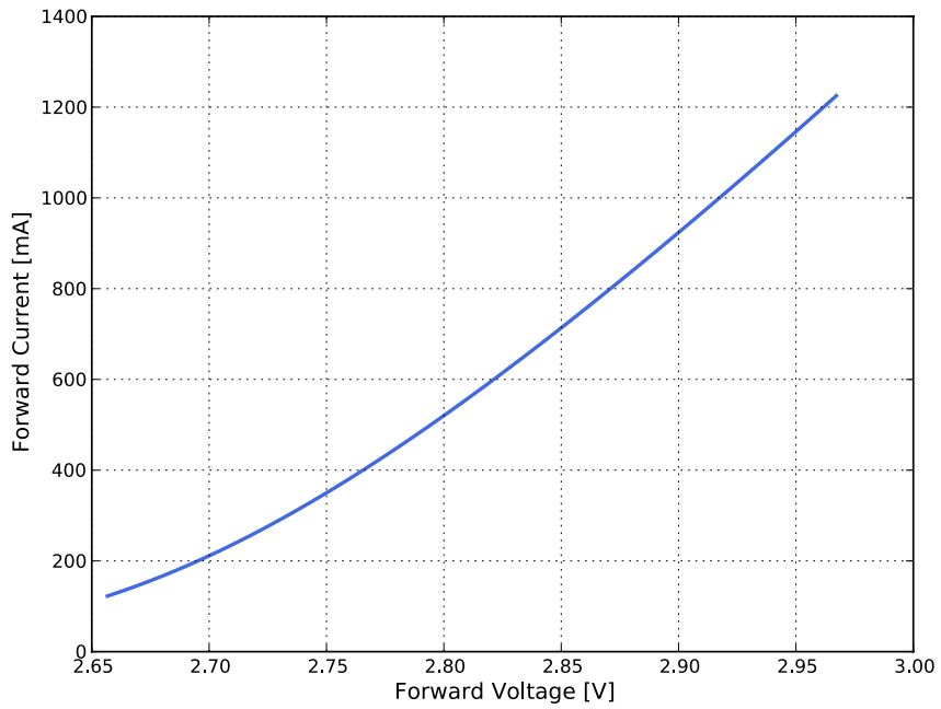
Figure 4f. Typical forward current vs. forward voltage for LUXEON CZ White at T_j=85^\circ\text{C} .
