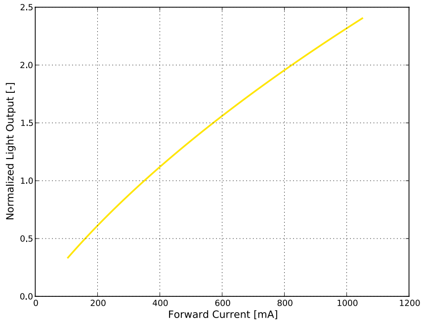
Figure 3b. Typical normalized light output vs. forward current for LUXEON CZ PC Amber at T_j=85^\circ\text{C} .
