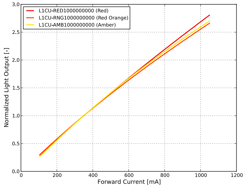
Figure 3a. Typical normalized light output vs. forward current for LUXEON CZ Red, Red-Orange and Amber at T_j=85^\circ\text{C} .
