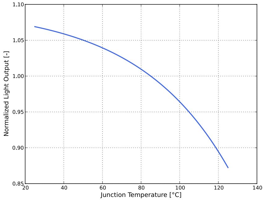
Figure 2f. Typical normalized light output vs. junction temperature for LUXEON CZ White at 350mA.
