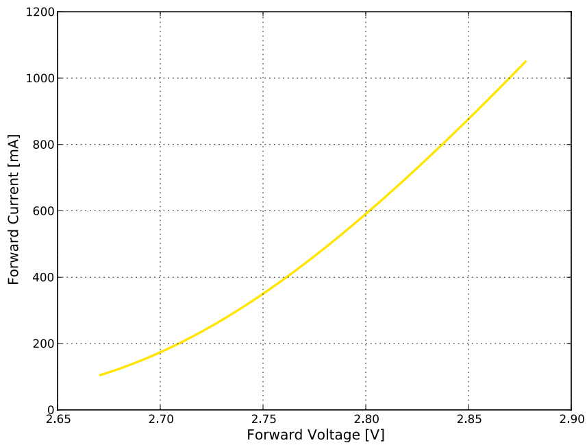
Figure 4b. Typical forward current vs. forward voltage for LUXEON CZ PC Amber at T_j=85^\circ\text{C} .
