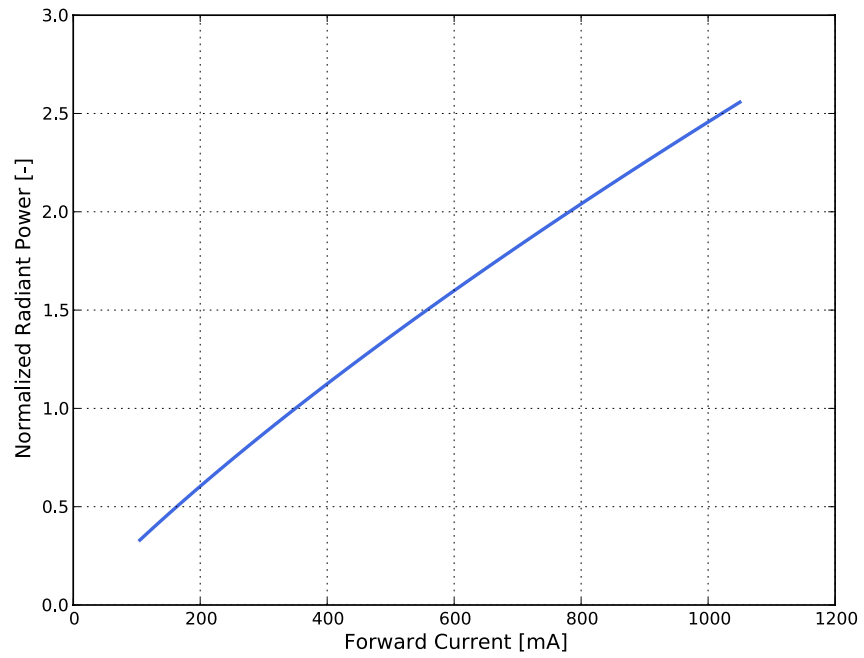
Figure 3e. Typical normalized radiant power vs. forward current for LUXEON CZ Royal Blue at T_j=85^\circ\text{C} .
