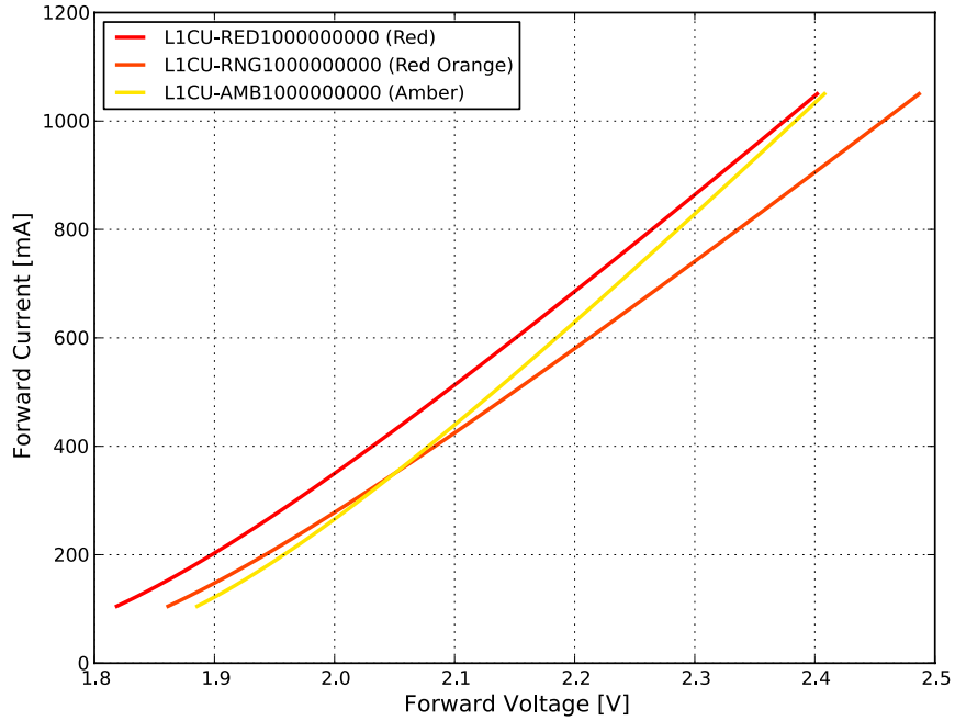
Figure 4a. Typical forward current vs. forward voltage for LUXEON CZ Red, Red-Orange and Amber at T_j=85^\circ\text{C} .
