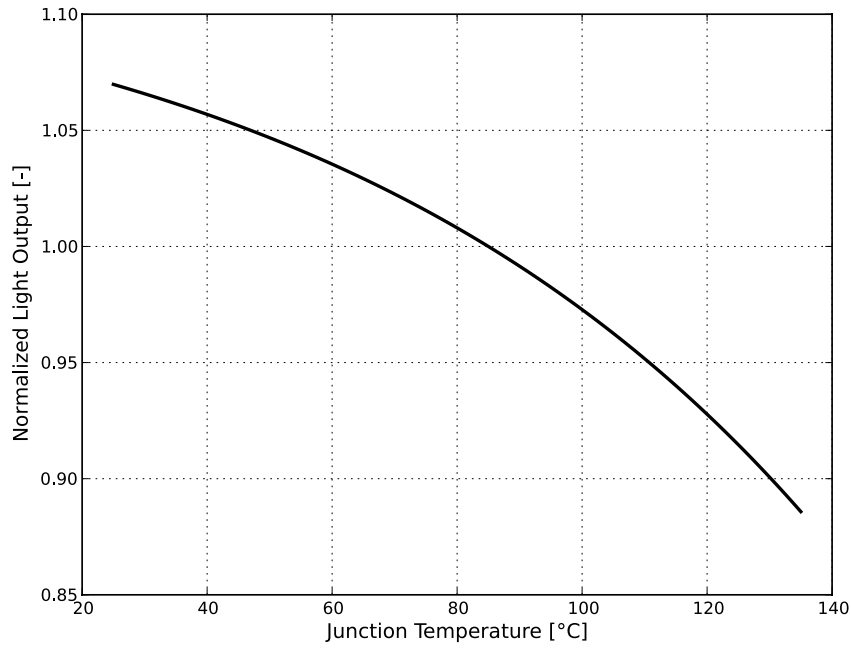
Figure 2c. Typical normalized light output vs. junction temperature for LUXEON CZ Mint at 350mA.
