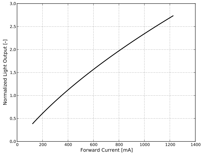
Figure 3c. Typical normalized light output vs. forward current for LUXEON CZ Mint at T_j=85^\circ\text{C} .
