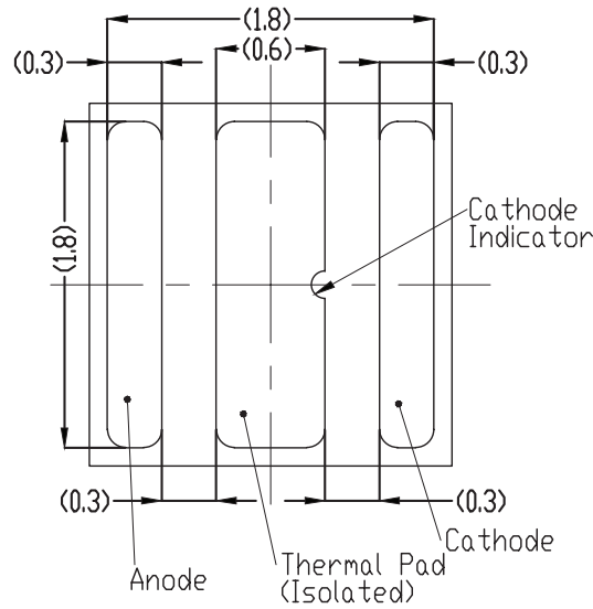
Figure 13. Recommended PCB solder pad layout for LUXEON CZ Color Line.
