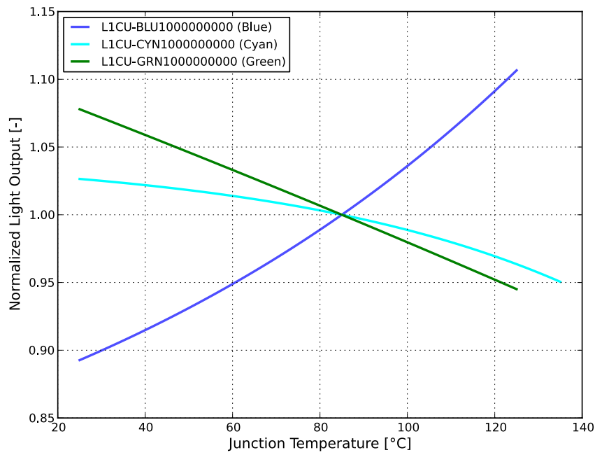
Figure 2d. Typical normalized light output vs. junction temperature for LUXEON CZ Green, Cyan and Blue at 350mA.
