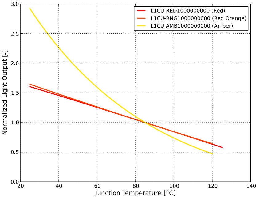
Figure 2a. Typical normalized light output vs. junction temperature for LUXEON CZ Red, Red-Orange and Amber at 350mA.
