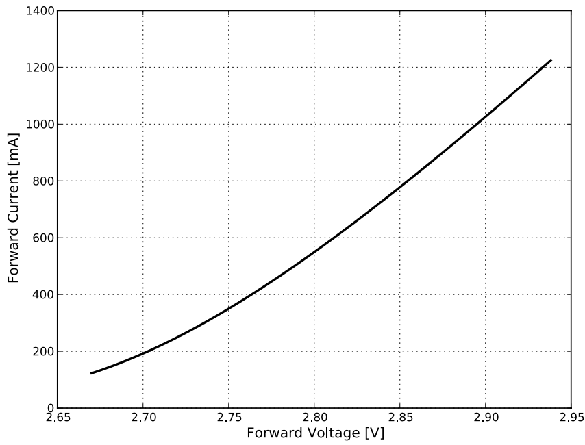
Figure 4c. Typical forward current vs. forward voltage for LUXEON CZ Mint at T_j=85^\circ\text{C} .
