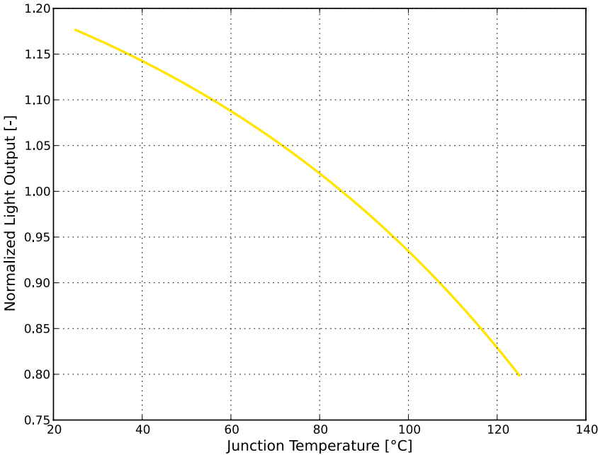
Figure 2b. Typical normalized light output vs. junction temperature for LUXEON CZ PC Amber at 350mA.
