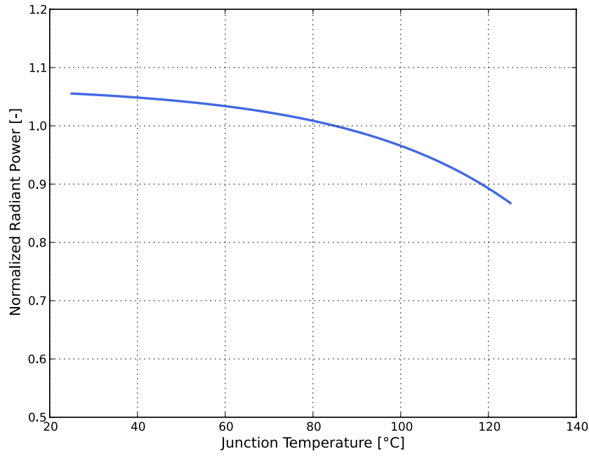
Figure 2e. Typical normalized radiant power vs. junction temperature for LUXEON CZ Royal Blue at 350mA.
