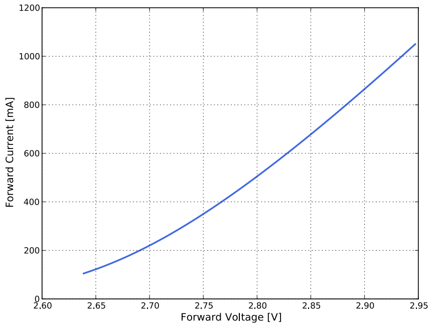
Figure 4e. Typical forward current vs. forward voltage for LUXEON CZ Royal Blue at T_j=85^\circ\text{C} .
