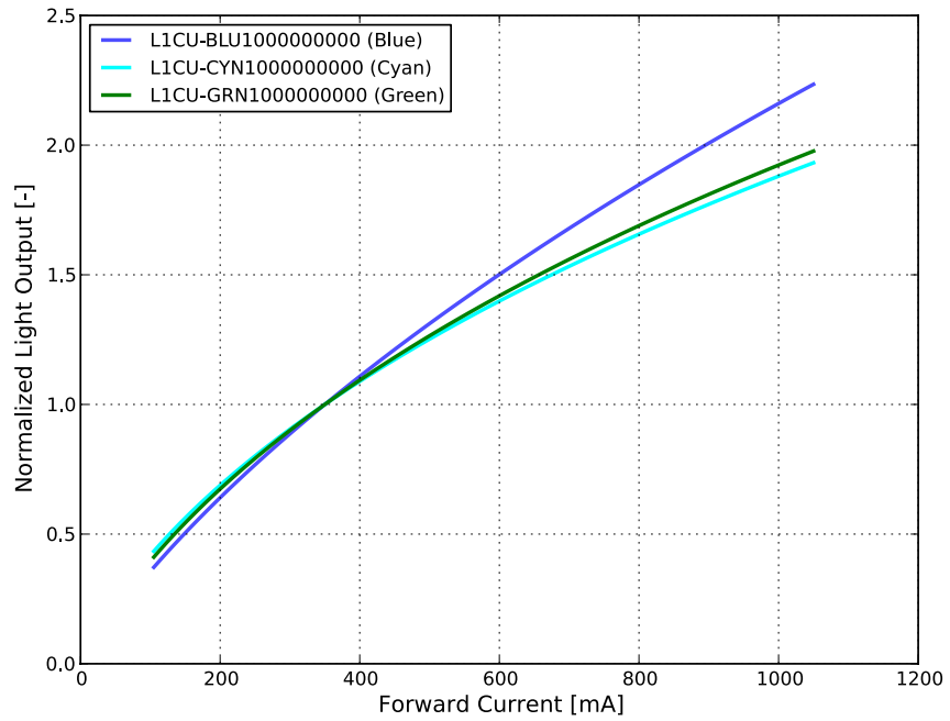
Figure 3d. Typical normalized light output vs. forward current for LUXEON CZ Green, Cyan and Blue at T_j=85^\circ\text{C} .
