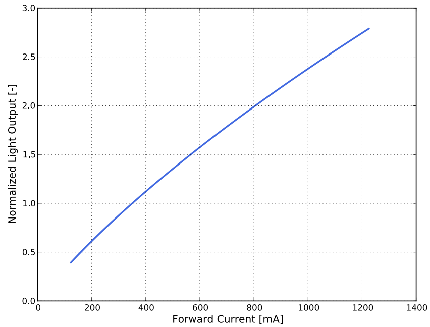
Figure 3f. Typical normalized light output vs. forward current for LUXEON CZ White at T_j=85^\circ\text{C} .
