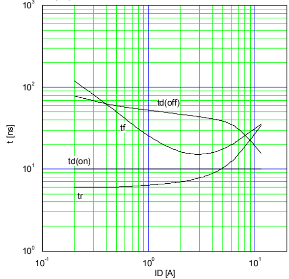
Typical Switching Characteristics vs. I D t=f(I_D):V_{cc}=300V, V_{GS}=10V, R_G=24\text{ }\Omega
