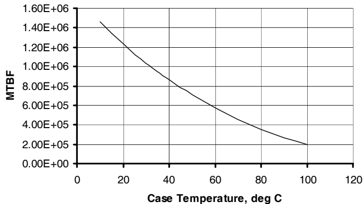
MTBF vs Case Temperature for AMR2803R3S
