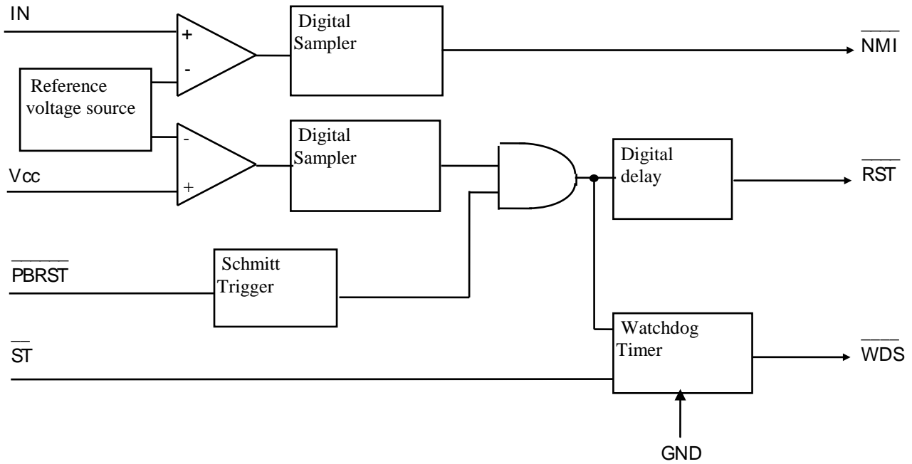
Fig. 8 – Block Diagram
