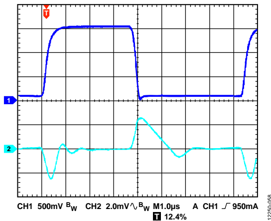
Figure 58. Output Transient Response, V_{OUT} = 5\text{ V} , C_{OUT} = 4.7\ \mu\text{F}
