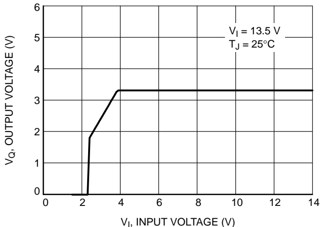
Figure 25. Output Voltage vs. Input Voltage
