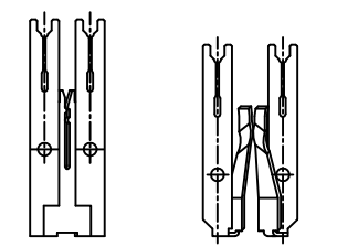
(CONNECTION) (DISCONNECTION)
