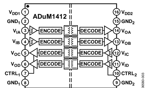
Figure 3. ADuM1412
