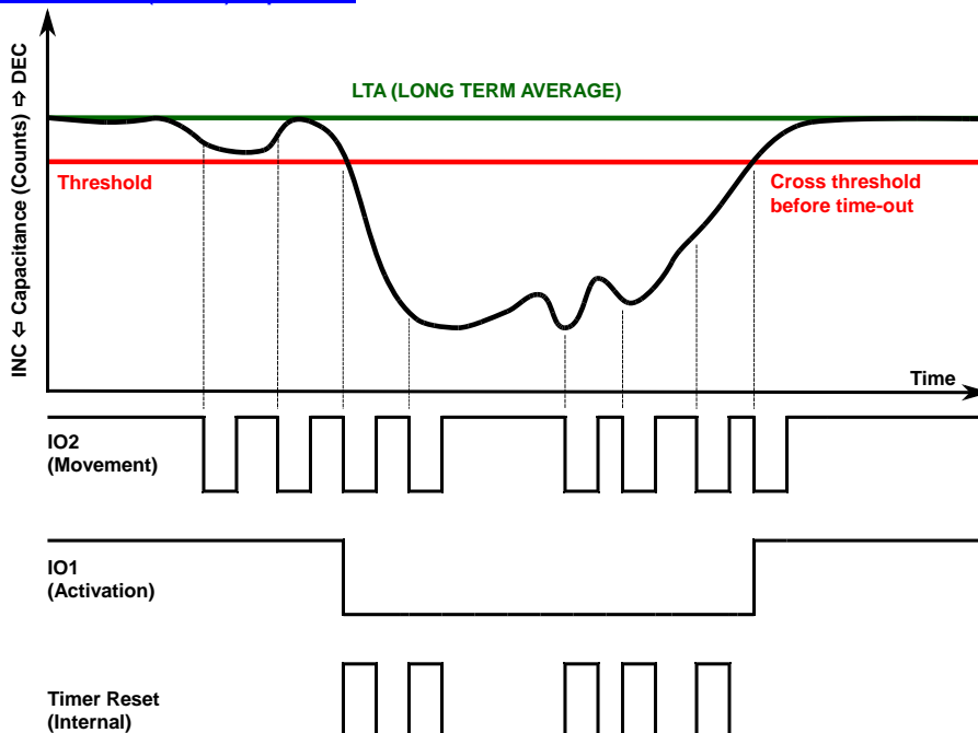
Figure 1.2 Plot of IQS211 streaming data along with the digital response
