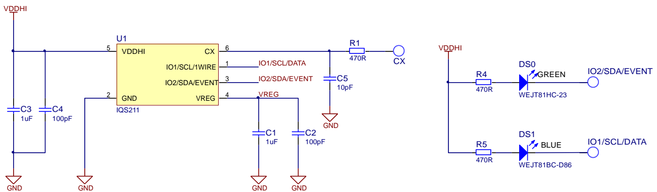
Figure 2.2 IQS211 reference schematic
