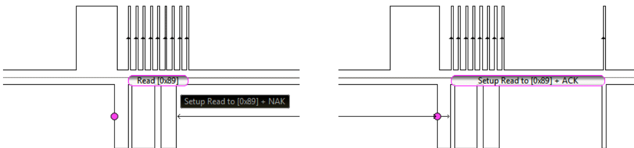
Figure 4.1 I2C polling examples: typical often repeated polling request with NACK (left) along with the successful request with ACK (right)
