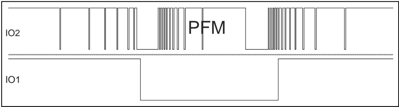
Figure 3.2 Movement (PFM) and activation output
