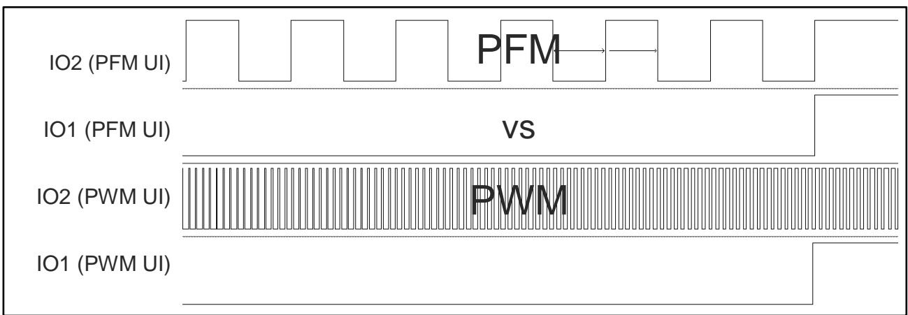
Figure 3.3 PFM movement output (TOP: 15ms period minimum) compared with PWM movement output (BOTTOM: 1ms period)
