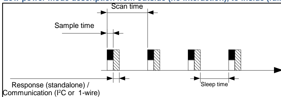
Figure 1.11 Low power mode description from outside (no interaction), to inside (full interaction)
