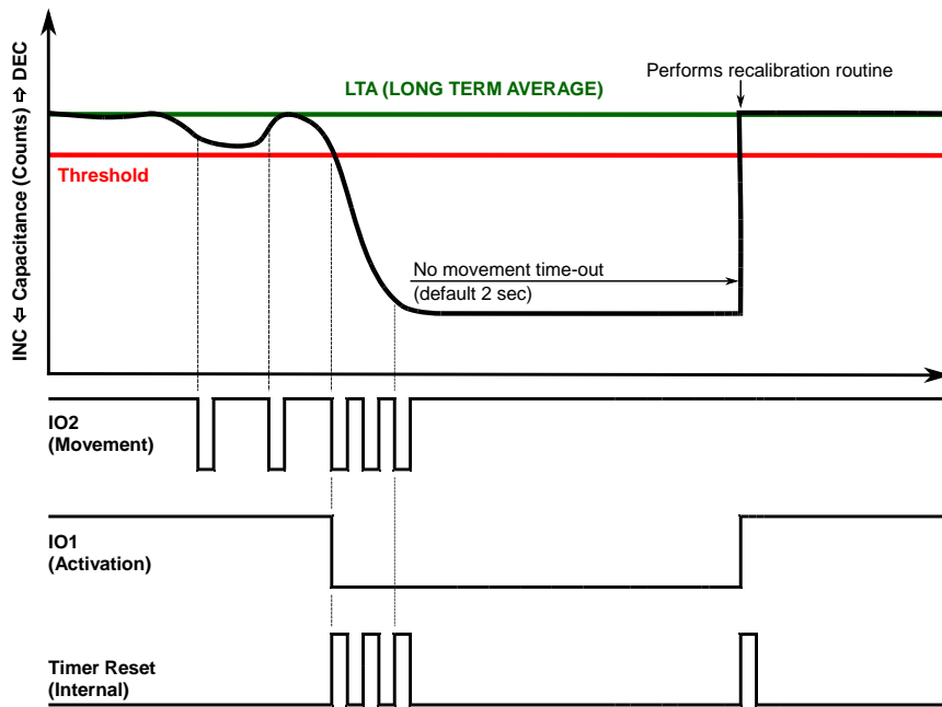
Figure 1.3 Example of a time-out event with re-calibration
