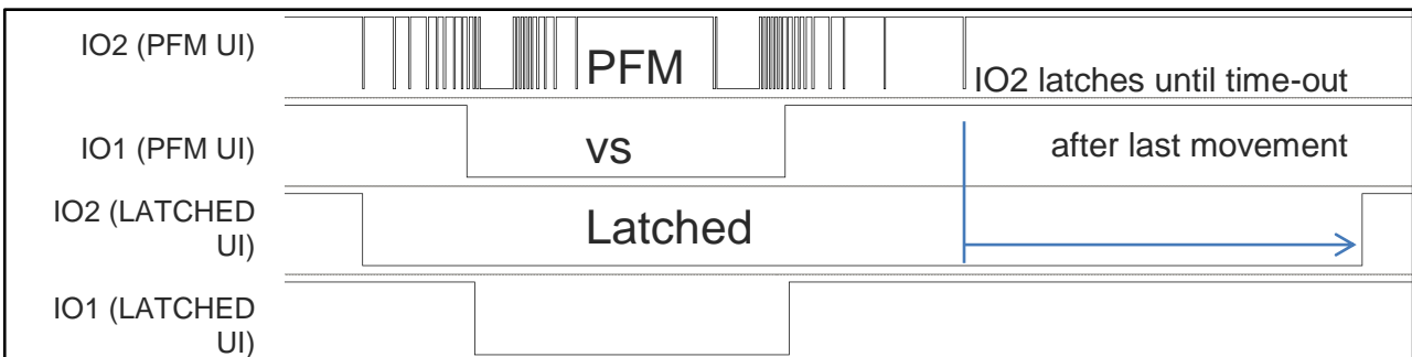
Figure 3.4 PFM movement output (TOP) compared with latched movement output (BOTTOM). Movement output is forced by first movement
