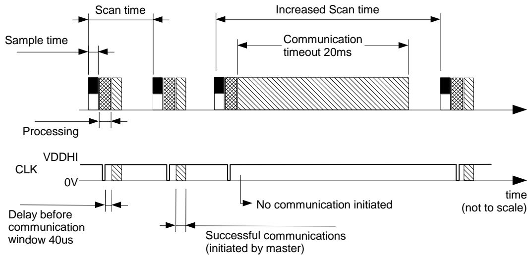
Figure 4.2 How to use RDY signal on clock line
