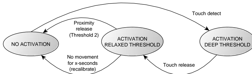
Figure 3.1 State diagram of touch late release interface
