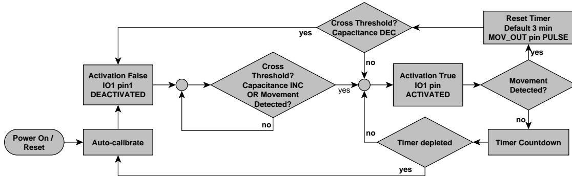
Figure 1.1 Flow diagram of the typical IQS211 movement based user interface
