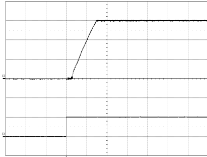
Start-up enabled by connecting V_i at: T_{ref} = +25^{\circ}\text{C} , V_i = 53\text{ V} , I_o = 30\text{ A} resistive load. Top trace: output voltage (0.5 V/div.). Bottom trace: input voltage (20 V/div.). Time scale: (5 ms/div.).
