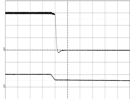
Shut-down enabled by disconnecting V_i at: T_{ref} = +25^{\circ}\text{C} , V_i = 53\text{ V} , I_o = 30\text{ A} resistive load. Top trace: output voltage (0.5 V/div.). Bottom trace: input voltage (50 V/div.). Time scale: (0.1 ms/div.).
