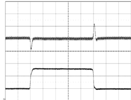
Output voltage response to load current step-change (7.5-22.5-7.5 A) at: T_{ref} = +25^{\circ}\text{C} , V_i = 53\text{ V} . Top trace: output voltage (200 mV/div.). Bottom trace: load current (10 A/div.). Time scale: (0.1 ms/div.).
