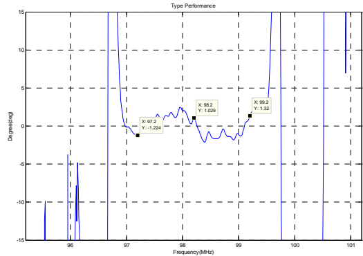
Phase Linearity (f0±1MHz)
