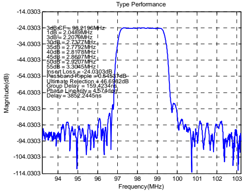
Frequency Response
