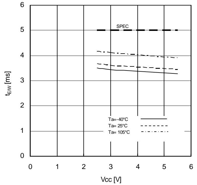
Figure 30. Write Cycle Time vs Supply Voltage
