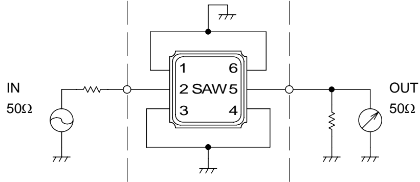
Fig.1 Measuring circuit
