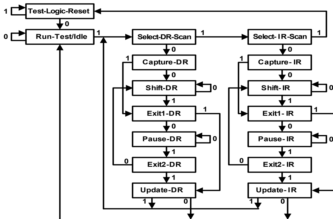
Figure 15. TAP Controller State Diagram
