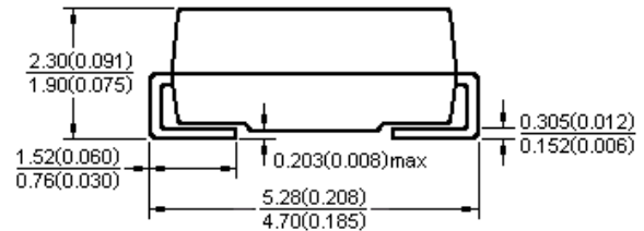
Dimintions in millimeters and (inchs)
