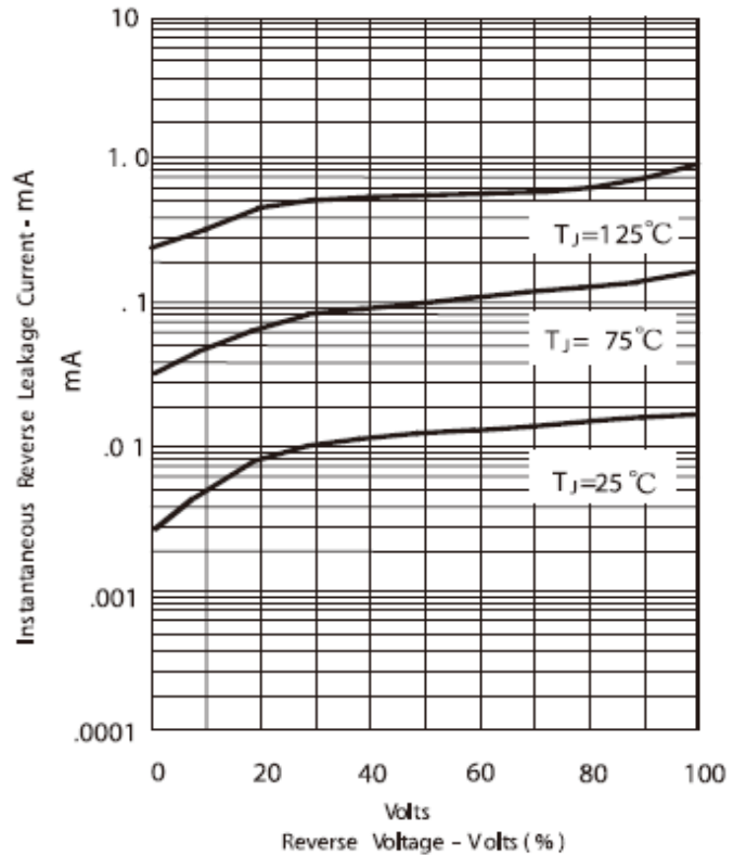
Figure 4-Typical Reverse Characteristics
