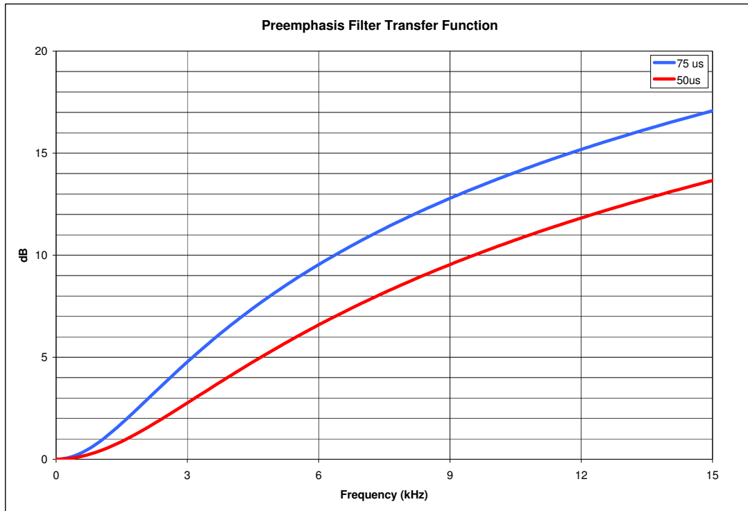
Figure 32. Pre-emphasis Filter Response
