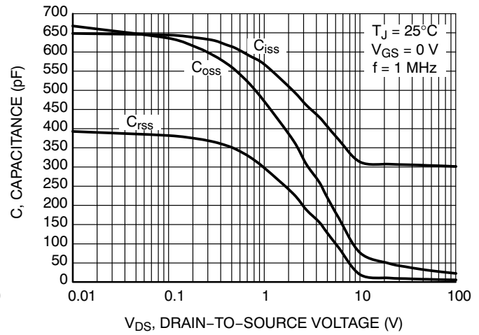
Figure 8. Capacitance Variation
