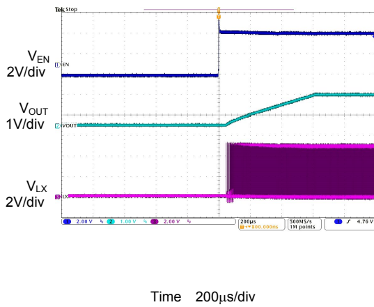
Figure 18. Soft Start
