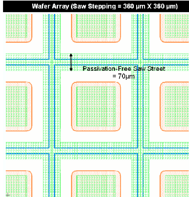
Figure 2. Wafer Array
