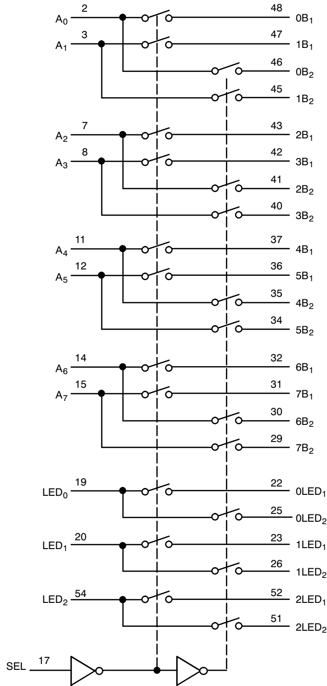
Figure 2. Block Diagram
