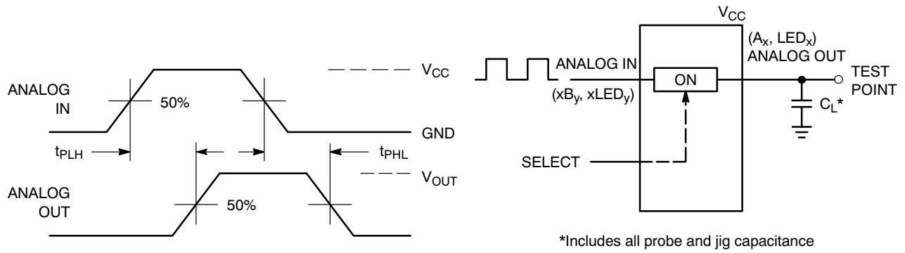
Figure 3. Propagation Delay
