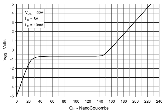
Fig. 14. Gate Charge
