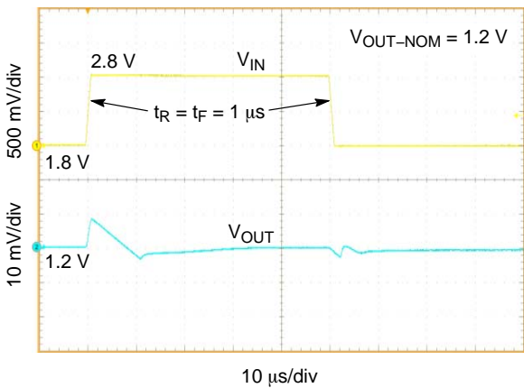
Figure 30. Line Transient Response
