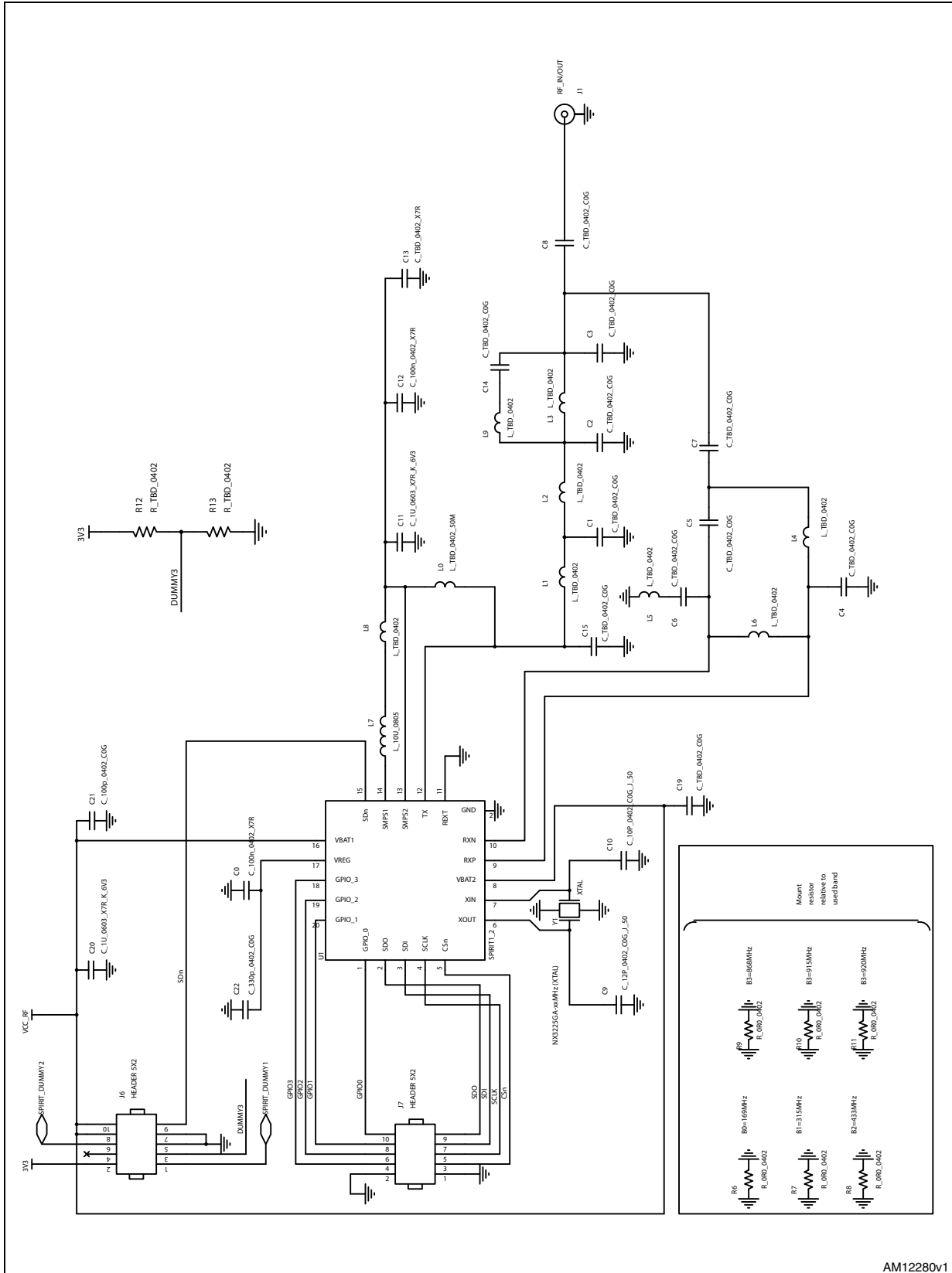
Figure 3. Daughterboard schematic
