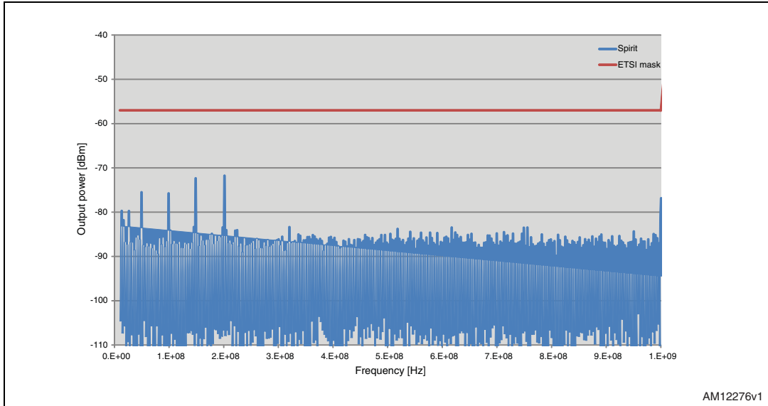
Figure 13. Receiver spurious emission below 1 GHz
