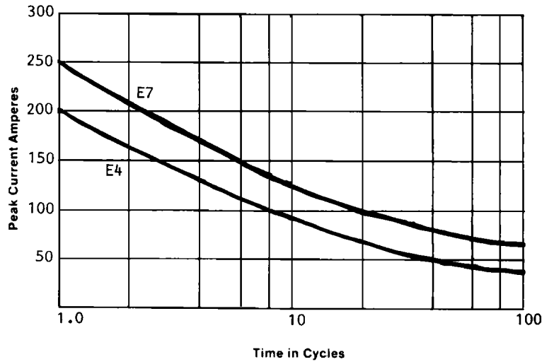
Surge Current at Rated Load
