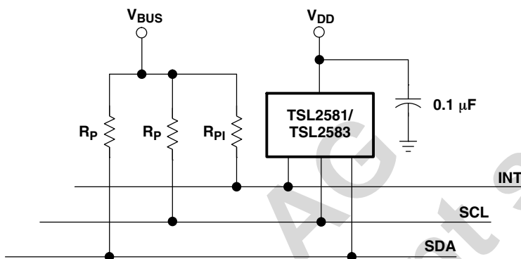
Figure 7. Bus Pull-Up Resistors
