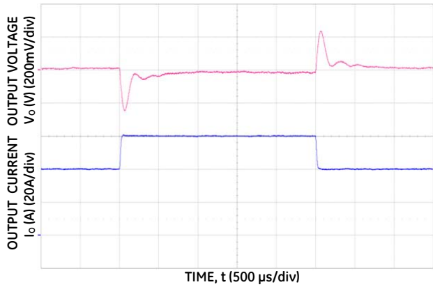
Figure 4. Typical Transient Response to 1A/ \mu s Step Change in Load from 50% to 75% to 50% of Full Load, C_o = 3200\mu F and 48 V dc Input.
