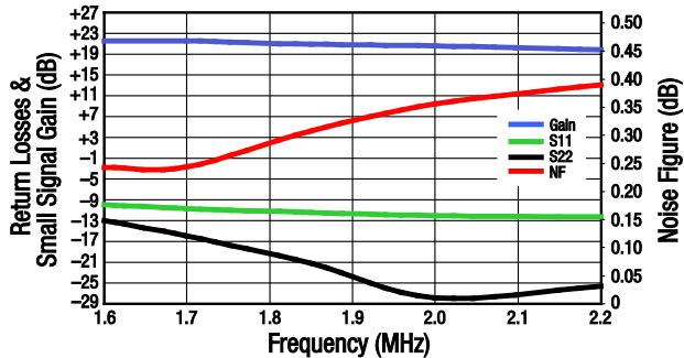
Figure 17. Evaluation Board NF, Gain, and Return Losses for 1600 to 2200 MHz Tuning
