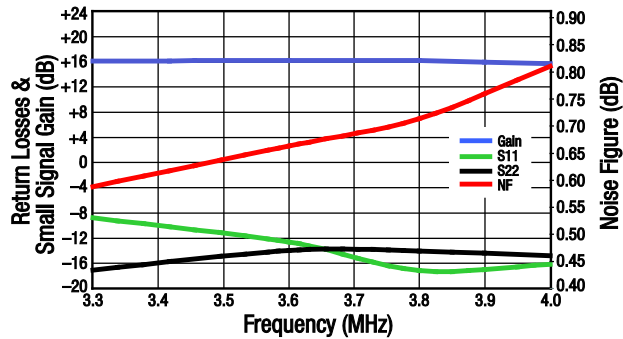
Figure 18. Evaluation Board NF, Gain, and Return Losses for 3400 to 3800 MHz Tuning
