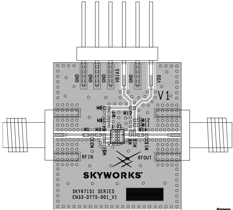
Figure 22. SKY67151-396LF Evaluation Board Assembly Diagram
