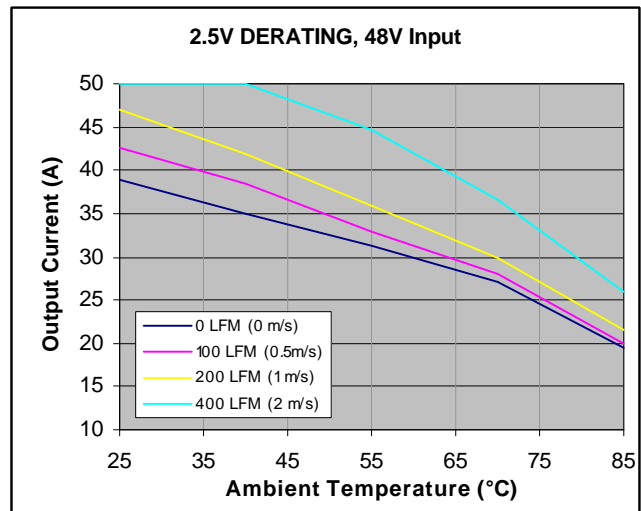
Figure 22. ALQ50G48 (2.5V) Output Derating curves at various airflow conditions directed across PIN 3 to 1 with the module mounted vertically.
