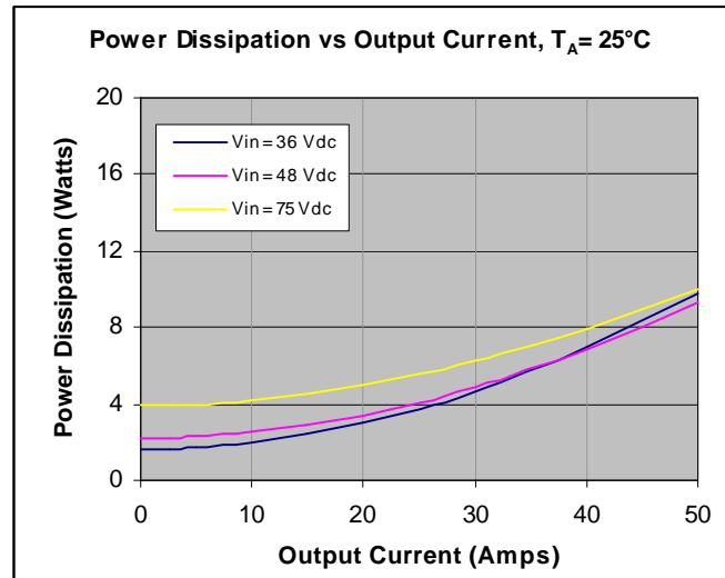
Figure 18. Power Dissipation vs. Load Current at T_A=25^\circ\text{C} for different input voltages with 300 LFM airflow directed from Pins 3 to 1.
