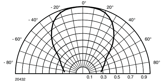
20432 Fig. 12 - Directivity
