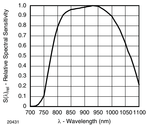
20431 Fig. 11 - Relative Spectral Sensitivity vs. Wavelength
