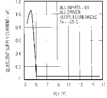
MAX621 QUIESCENT SUPPLY CURRENT vs. VCC
