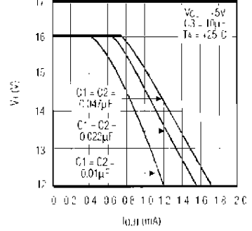
MAX620 V+ vs. IOUT
