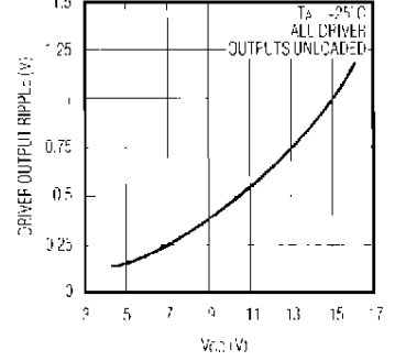
MAX621 DRIVER OUTPUT RIPPLE vs. VCC
