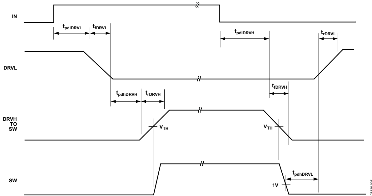
Figure 3. Timing Diagram
