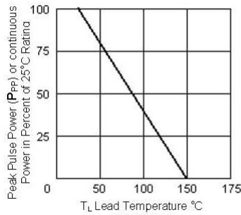
FIGURE 3 Derating Curve
