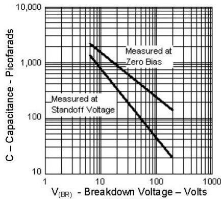
FIGURE 4 P5KE Typical Capacitance vs. Breakdown Voltage
