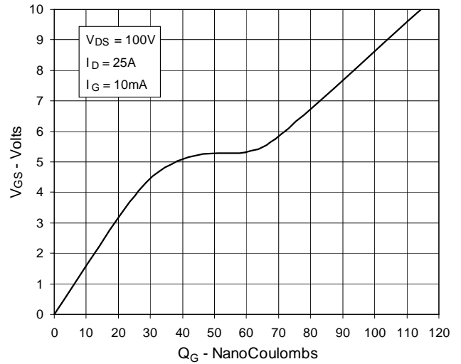
Fig. 10. Gate Charge
