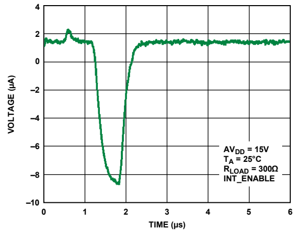
Figure 25. Output Current vs. Time on Output Enable
