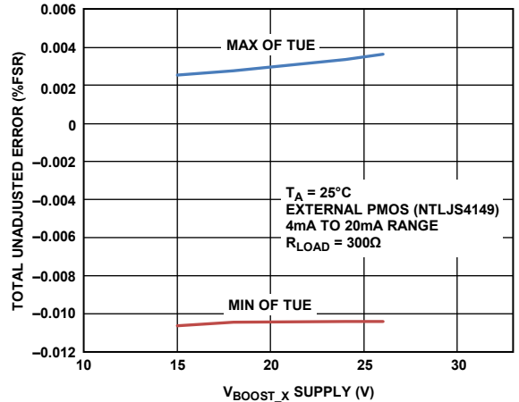
Figure 23. Total Unadjusted Error vs. V_{BOOST\_X} Using External PMOS Mode
