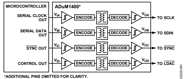
Figure 65. Isolated Interface
