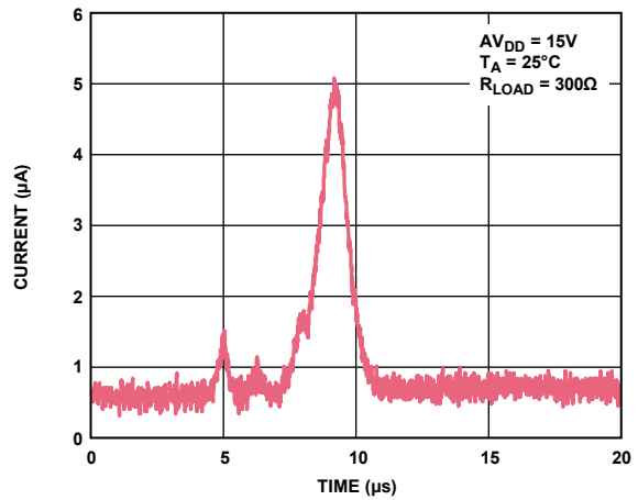
Figure 24. Output Current vs. Time on Power-Up
