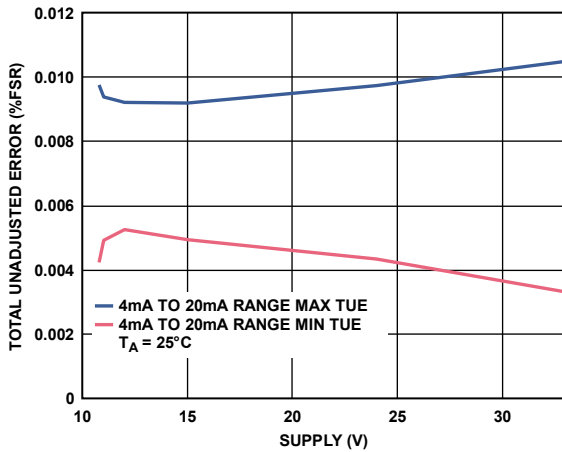
Figure 21. Total Unadjusted Error vs. AV_{DD} , External R_{SET}
