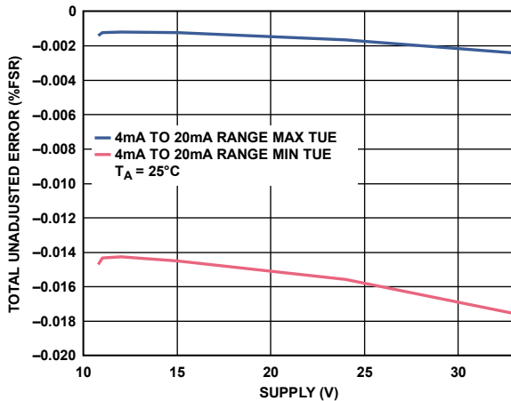
Figure 22. Total Unadjusted Error vs. AV_{DD} , Internal R_{SET}
