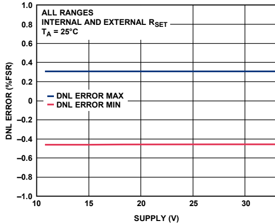
Figure 20. Differential Nonlinearity Error vs. AV_{DD}
