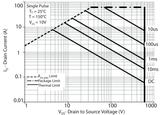
Maximum Rate Forward Biased Safe Operating Area
