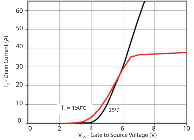
Transfer Characteristics
