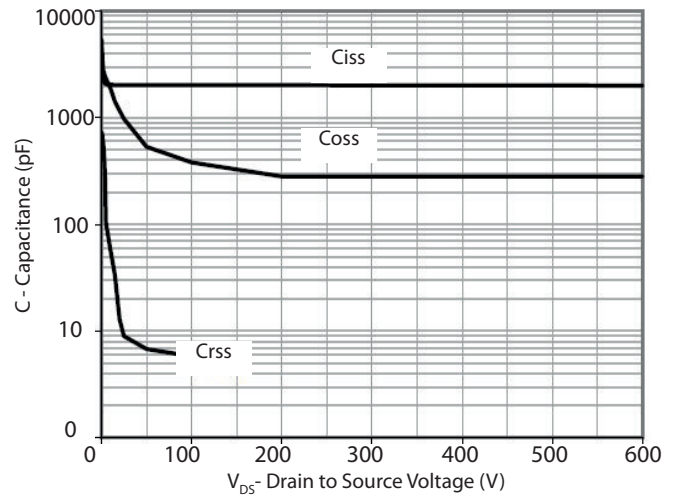
Capacitance
