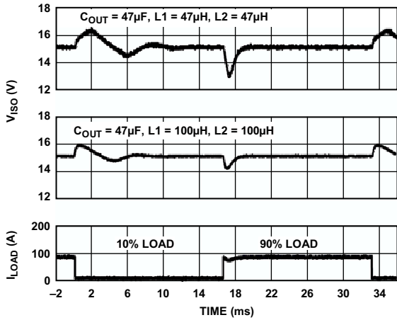
Figure 33. Typical V_{iso} Load Transient Response at 10% to 90% of 100 mA Load, f_{sw} = 500 kHz, 5 V Input to 15 V Output
