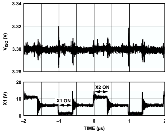
Figure 35. Typical V_{iso} Output Voltage Ripple at 400 mA Load, f_{sw} = 500 kHz, 5 V Input to 3.3 V Output
