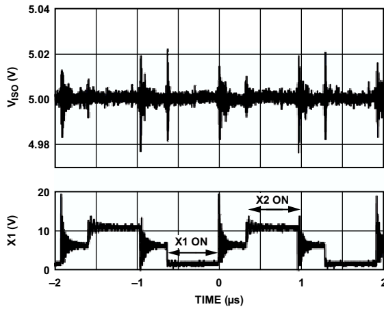
Figure 34. Typical V_{iso} Output Voltage Ripple at 400 mA Load, f_{sw} = 500 kHz, 5 V Input to 5 V Output
