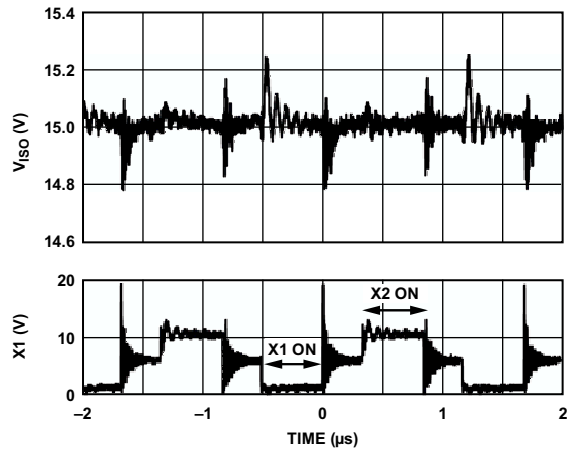
Figure 37. Typical V_{iso} Output Voltage Ripple at 100 mA Load, f_{sw} = 500 kHz, 5 V Input to 15 V Output
