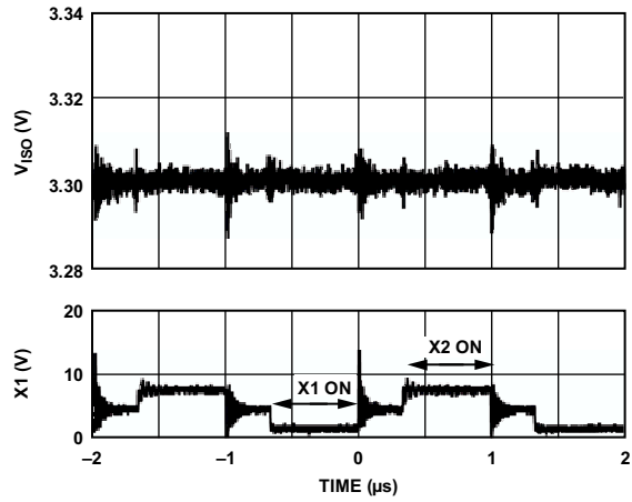
Figure 36. Typical V_{iso} Output Voltage Ripple at 250 mA Load, f_{sw} = 500 kHz, 3.3 V Input to 3.3 V Output
