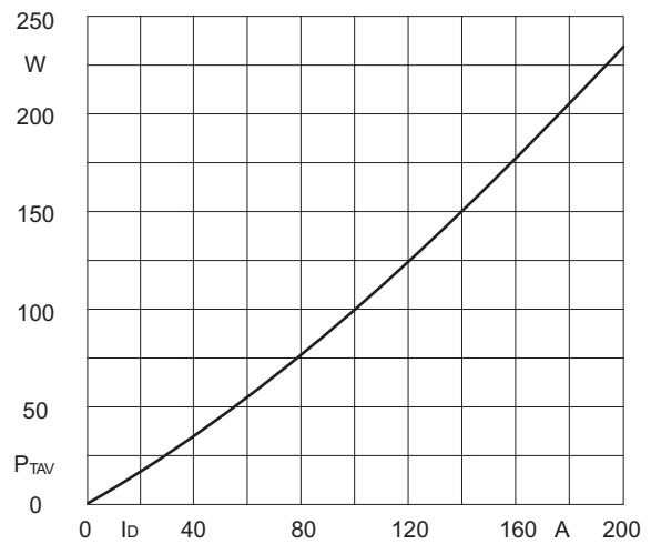
Fig.6 SCR power dissipation
