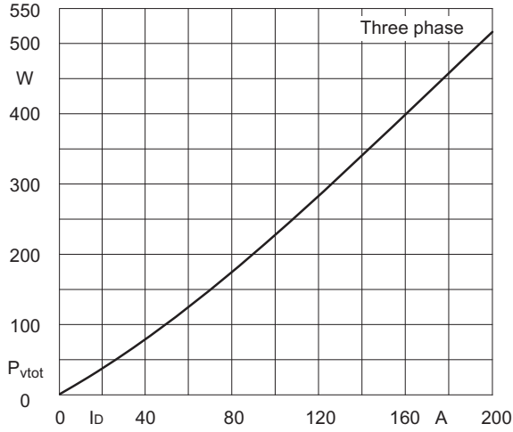
Fig.1 Power dissipation
