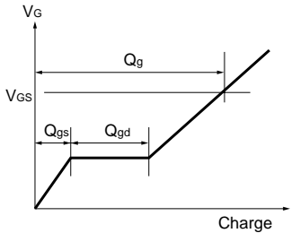
Fig.14 Gate Charge Waveform
