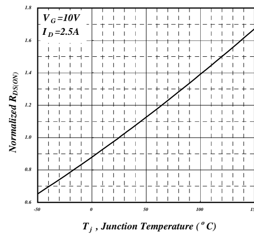
Fig 4. Normalized On-Resistance
