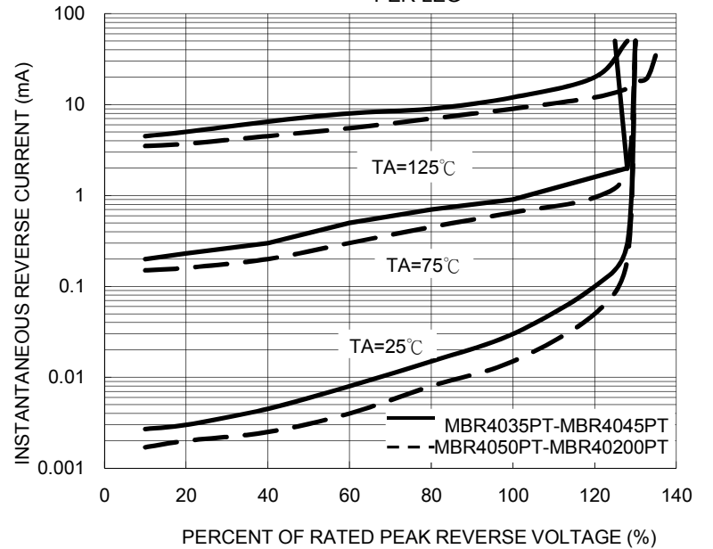
FIG.4 TYPICAL REVERSE CHARACTERISTICS PER LEG
