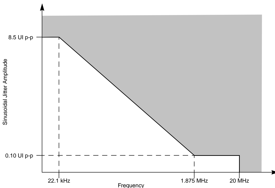
Figure 30. Single Frequency Sinusoidal Jitter Limits
