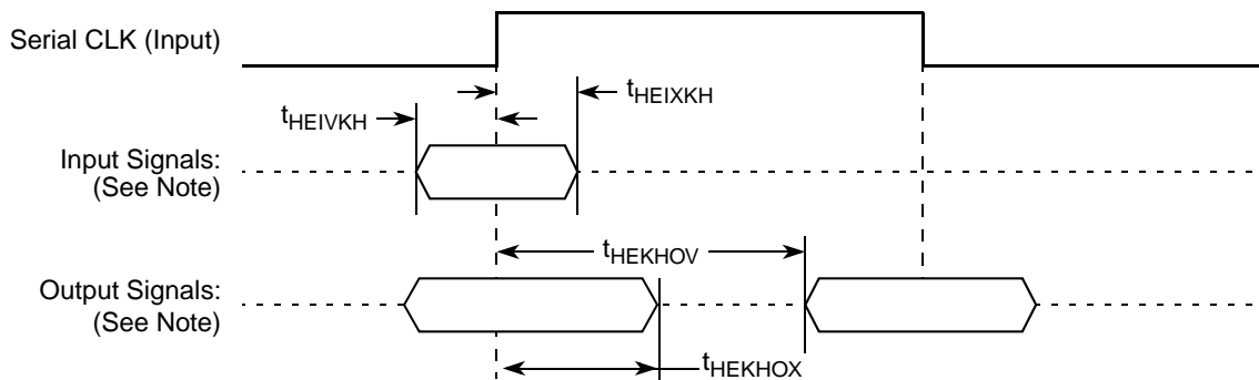
Figure 36. AC Timing (External Clock) Diagram
