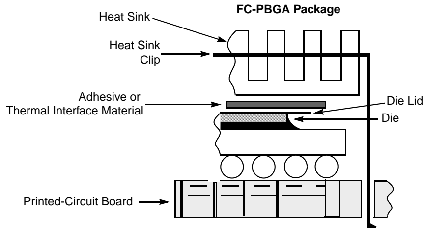
Figure 73. Package Exploded Cross-Sectional View
