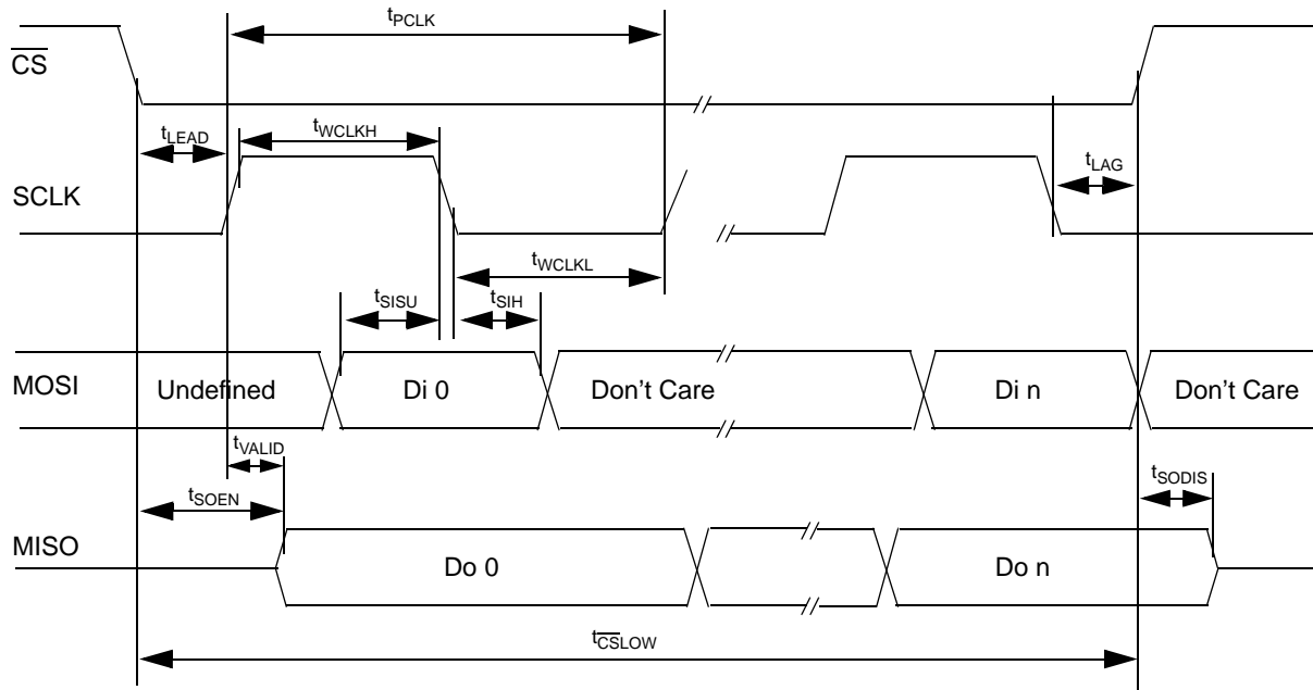
Figure 14. SPI Timings
