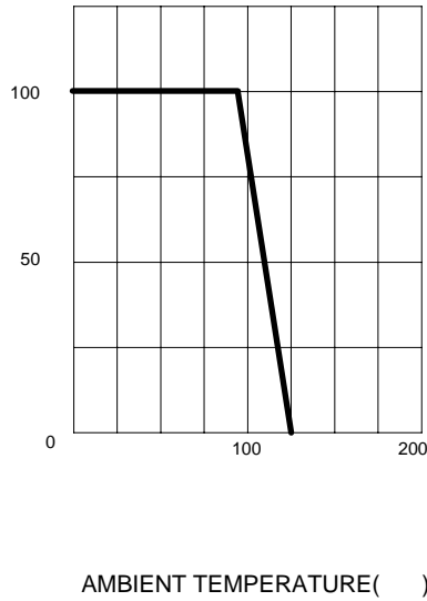
FIG.1 – ADMISSIBLE POWER DISSIPATION VS. AMBIENT TEMPERATURE
